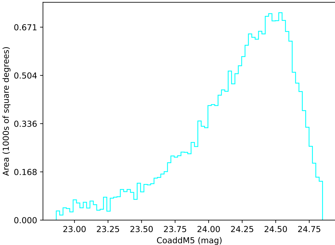
weather_cloudso0v3.5_10yrs Yr 3-4 u band: CoaddM5
