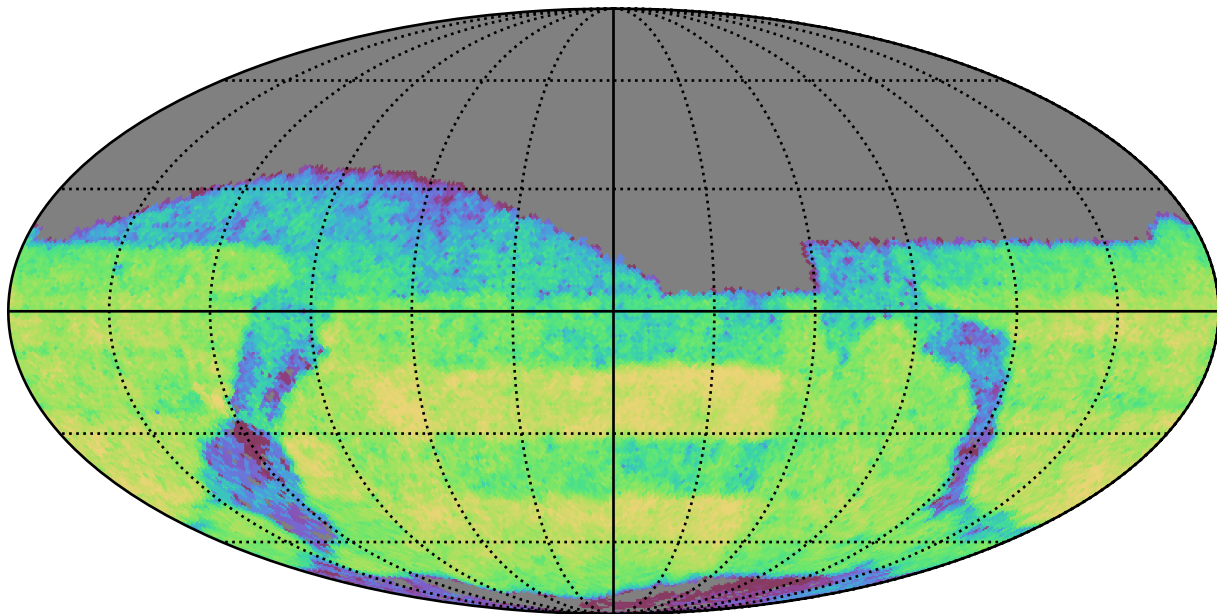
weather_cloudso0v3.5_10yrs Yr 3-4 i band: CoaddM5
