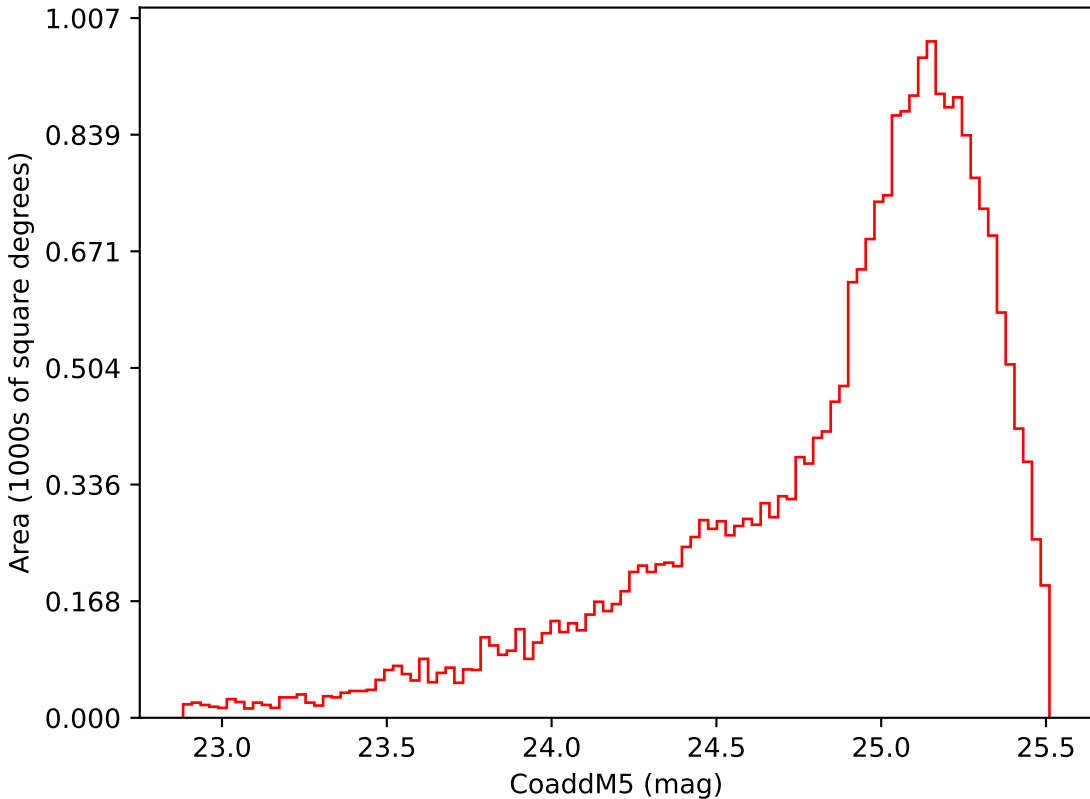
weather_cloudso0v3.5_10yrs Yr 3-4 i band: CoaddM5
