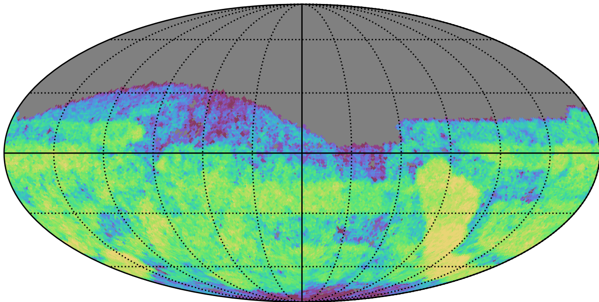
weather_cloudso0v3.5_10yrs Yr 3-4 g band: CoaddM5
