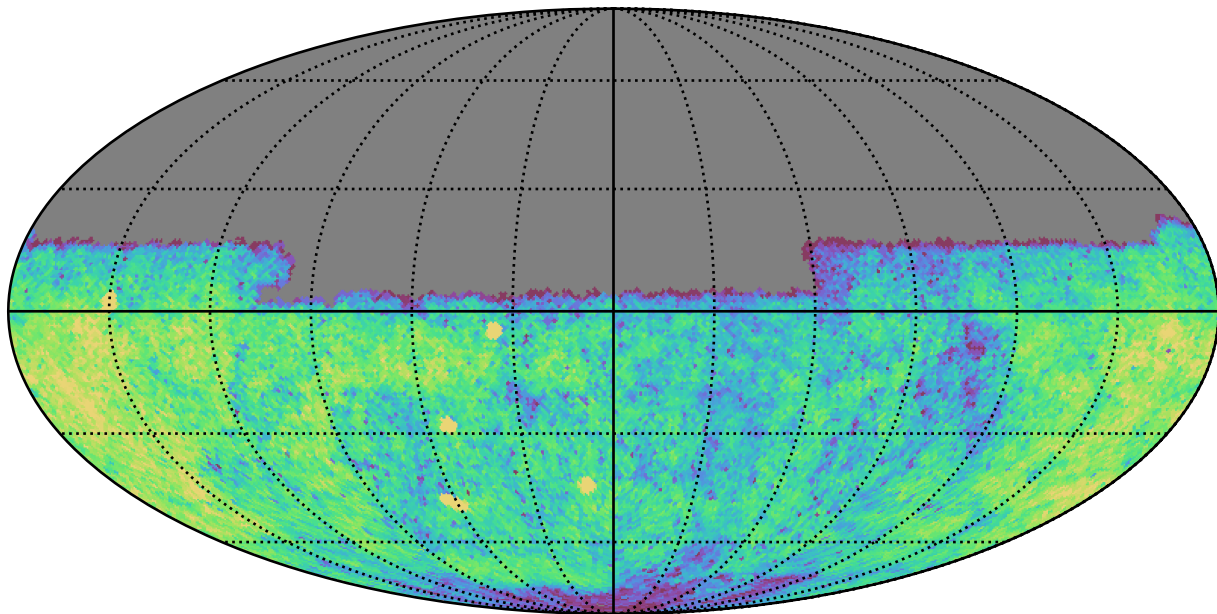
weather_cloudso0v3.5_10yrs Yr 1 u band: CoaddM5
