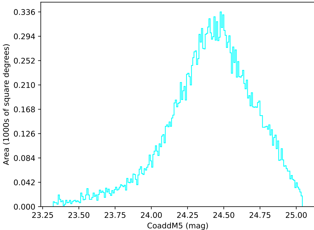
weather_cloudso0v3.5_10yrs Yr 1 u band: CoaddM5
