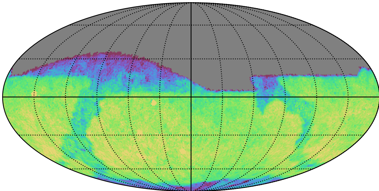
weather_cloudso0v3.5_10yrs Yr 1 r band: CoaddM5
