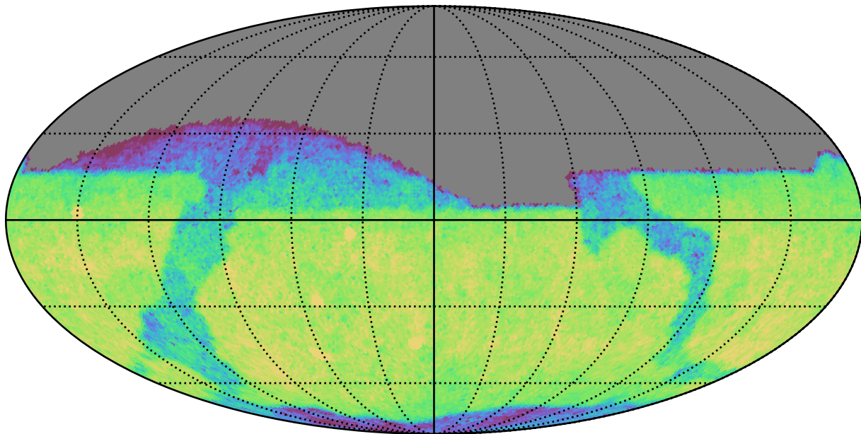
weather_cloudso0v3.5_10yrs Yr 1 i band: CoaddM5
