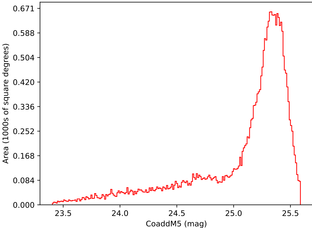
weather_cloudso0v3.5_10yrs Yr 1 i band: CoaddM5
