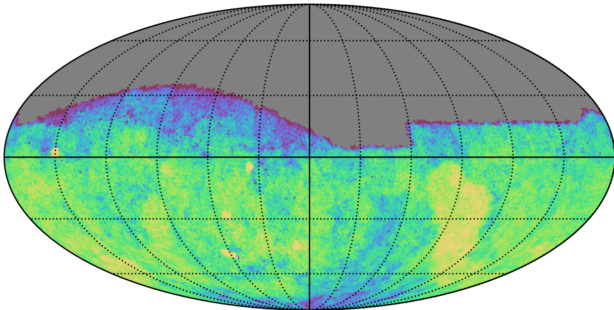
weather_cloudso0v3.5_10yrs Yr 1 g band: CoaddM5
