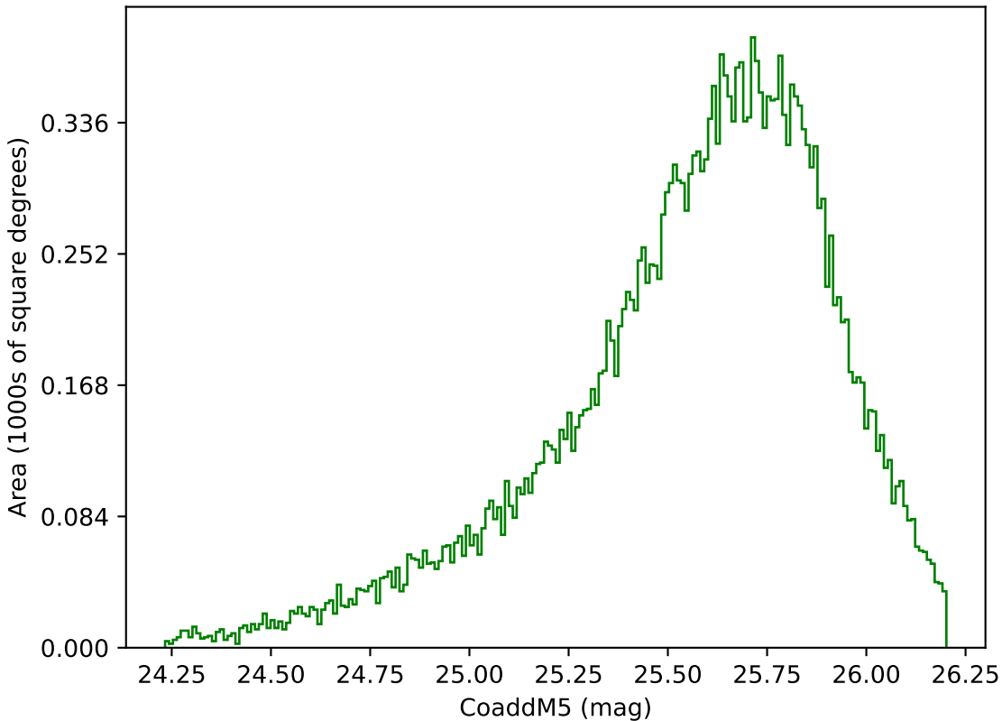
weather_cloudso0v3.5_10yrs Yr 1 g band: CoaddM5
