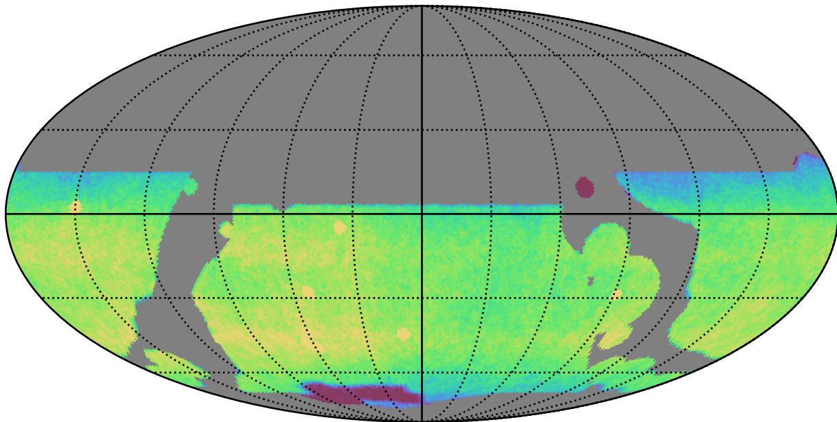
weather_cloudso0v3.5_10yrs WFD z band: CoaddM5
