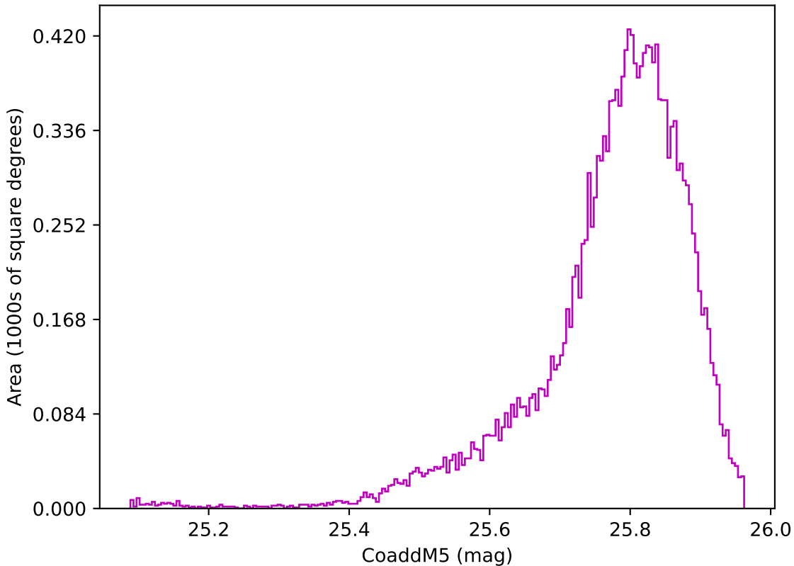
weather_cloudso0v3.5_10yrs WFD z band: CoaddM5
