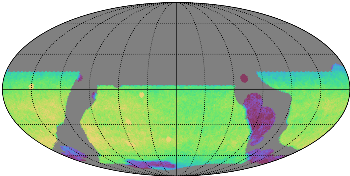
weather_cloudso0v3.5_10yrs WFD y band: CoaddM5
