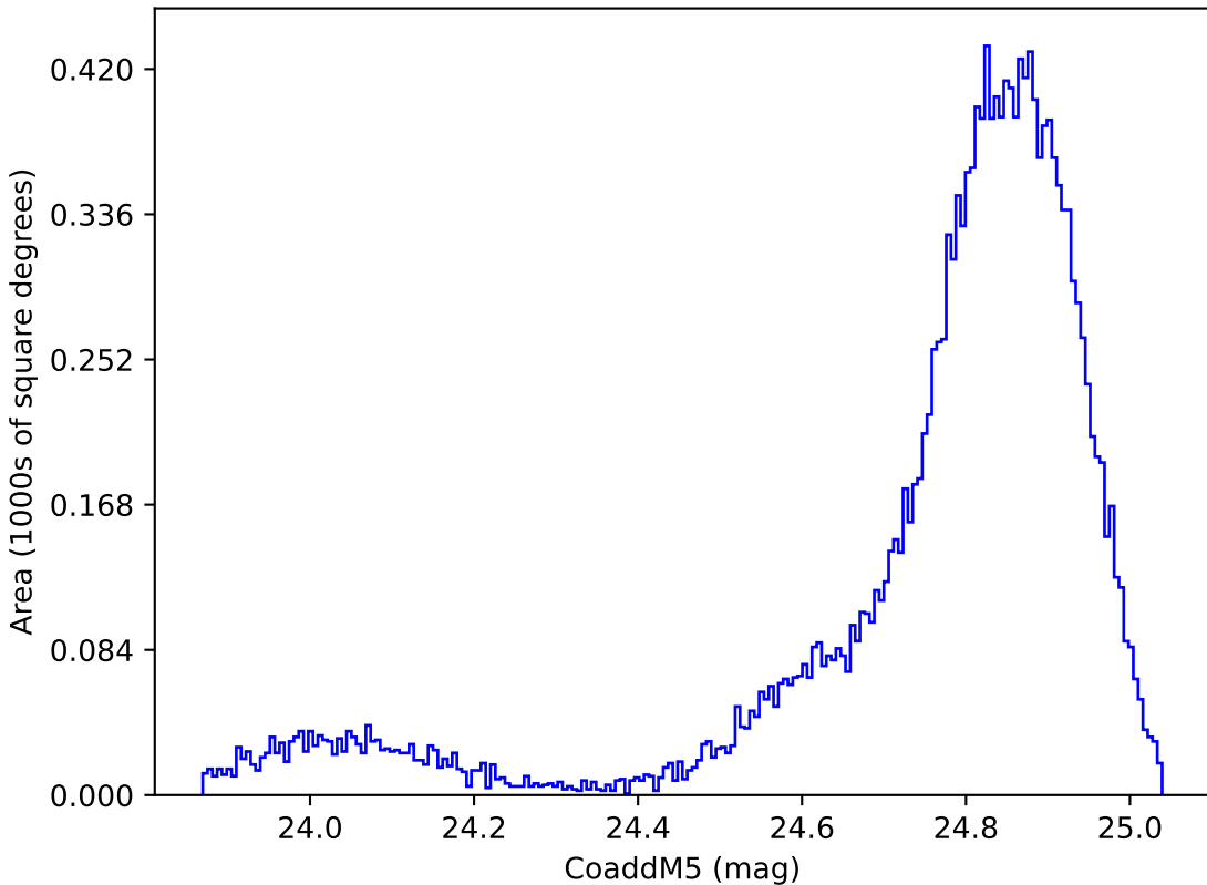
weather_cloudso0v3.5_10yrs WFD y band: CoaddM5
