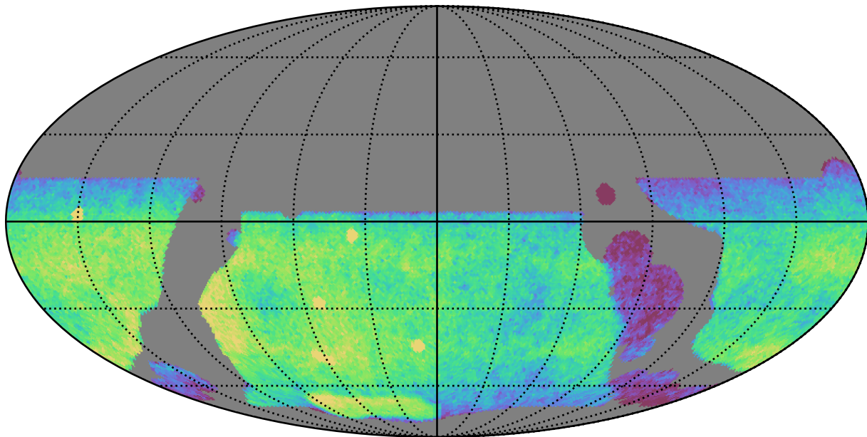
weather_cloudso0v3.5_10yrs WFD u band: CoaddM5
