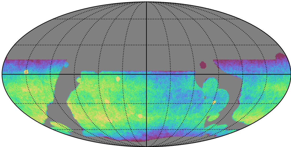
weather_cloudso0v3.5_10yrs WFD r band: CoaddM5
