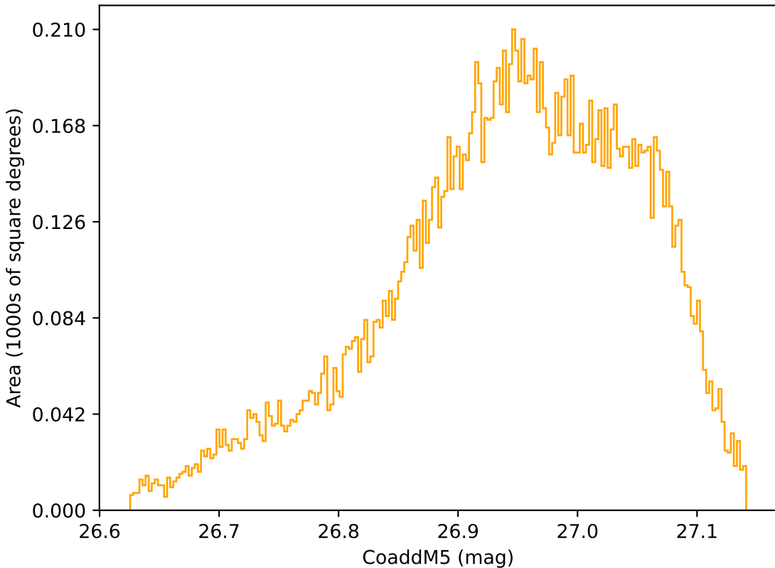
weather_cloudso0v3.5_10yrs WFD r band: CoaddM5
