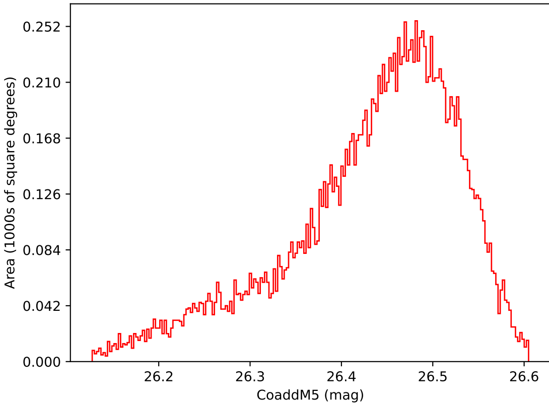
weather_cloudso0v3.5_10yrs WFD i band: CoaddM5
