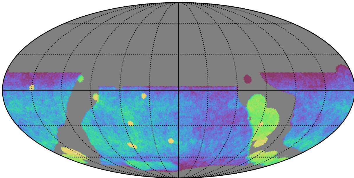
weather_cloudso0v3.5_10yrs WFD g band: CoaddM5
