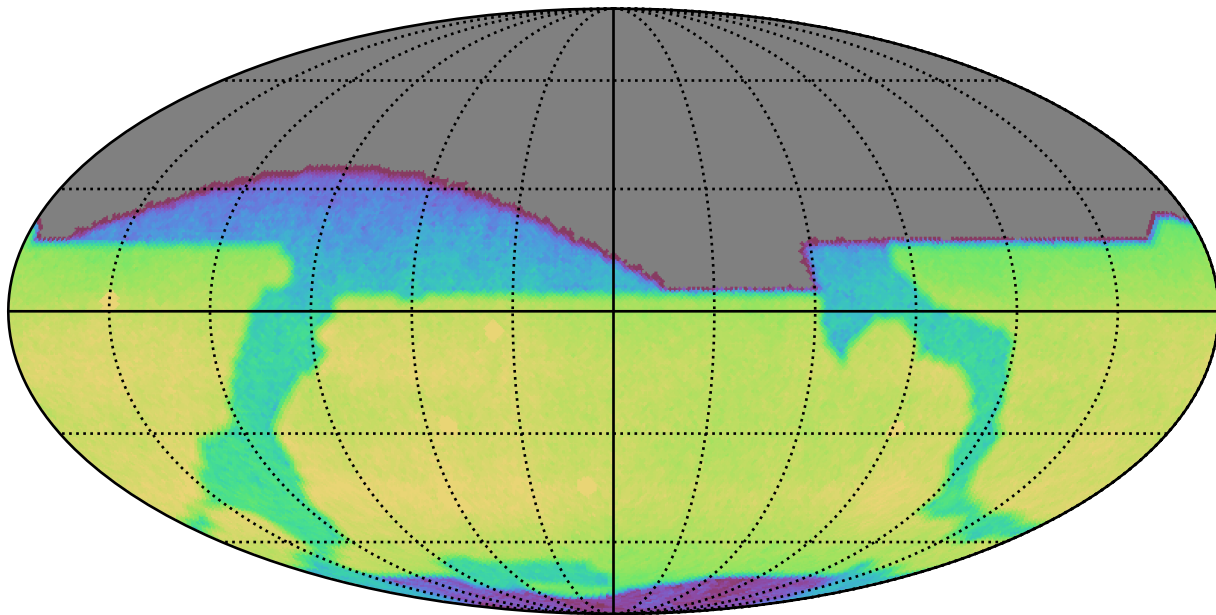
weather_cloudso0v3.5_10yrs All sky z band: CoaddM5
