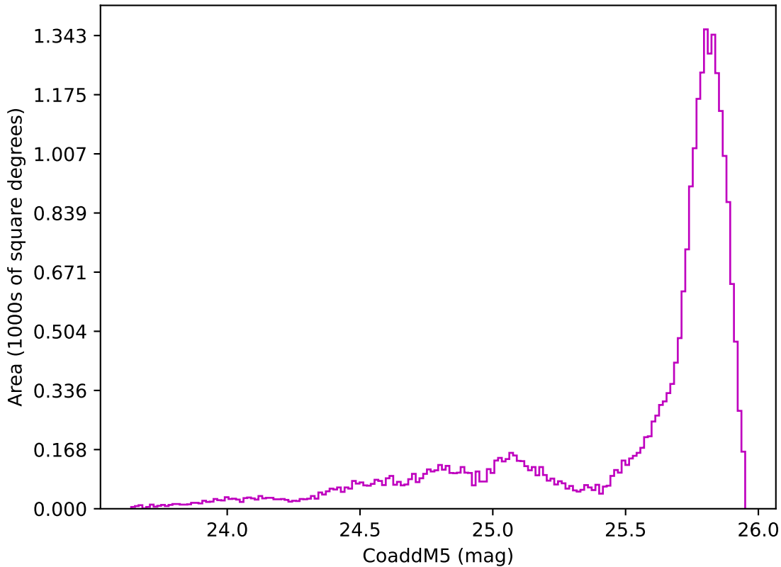
weather_cloudso0v3.5_10yrs All sky z band: CoaddM5
