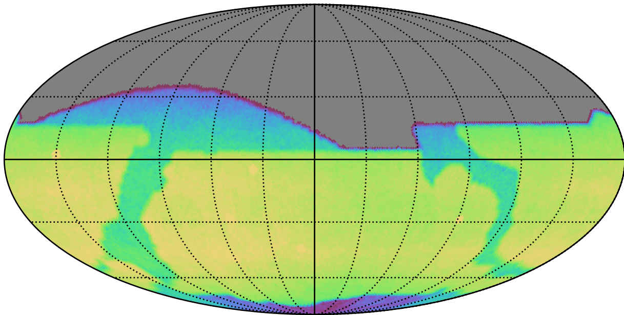
weather_cloudso0v3.5_10yrs All sky r band: CoaddM5
