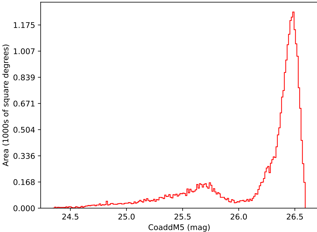
weather_cloudso0v3.5_10yrs All sky i band: CoaddM5
