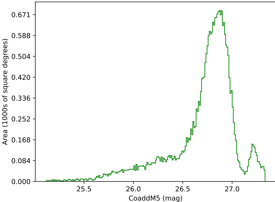
weather_cloudso0v3.5_10yrs All sky g band: CoaddM5
