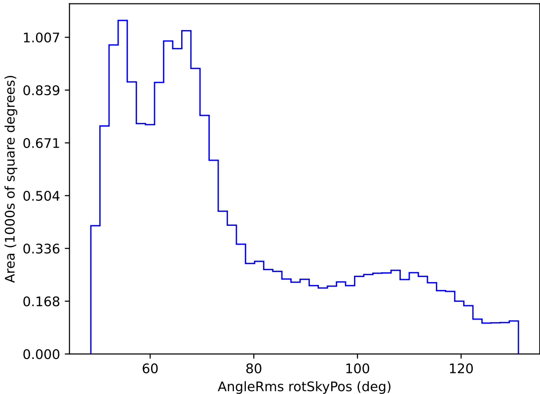
weather_cloudso0v3.5_10yrs WFD z band: AngleRms rotSkyPos
