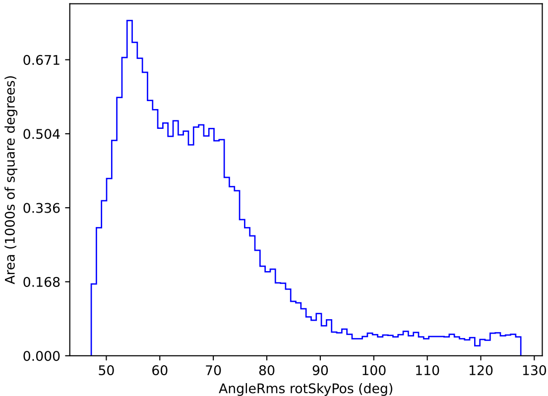
weather_cloudso0v3.5_10yrs WFD y band: AngleRms rotSkyPos
