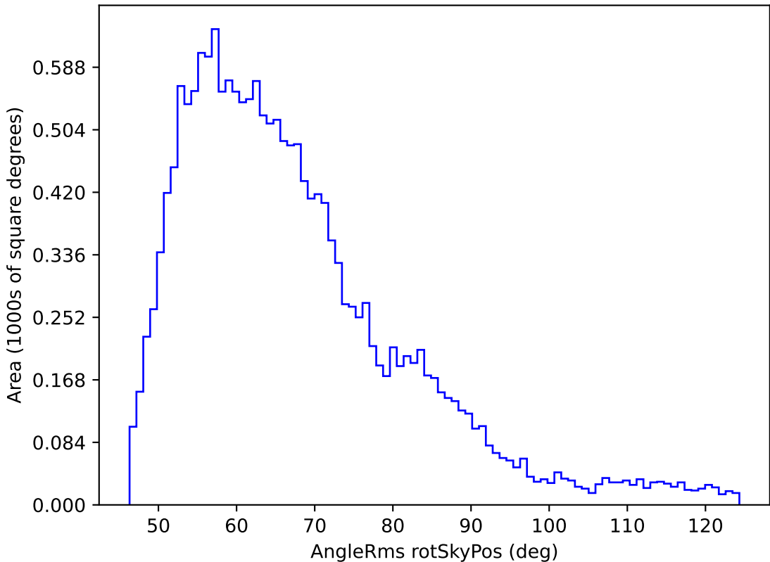
weather_cloudso0v3.5_10yrs WFD u band: AngleRms rotSkyPos
