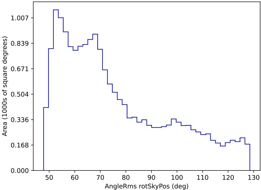
weather_cloudso0v3.5_10yrs WFD r band: AngleRms rotSkyPos
