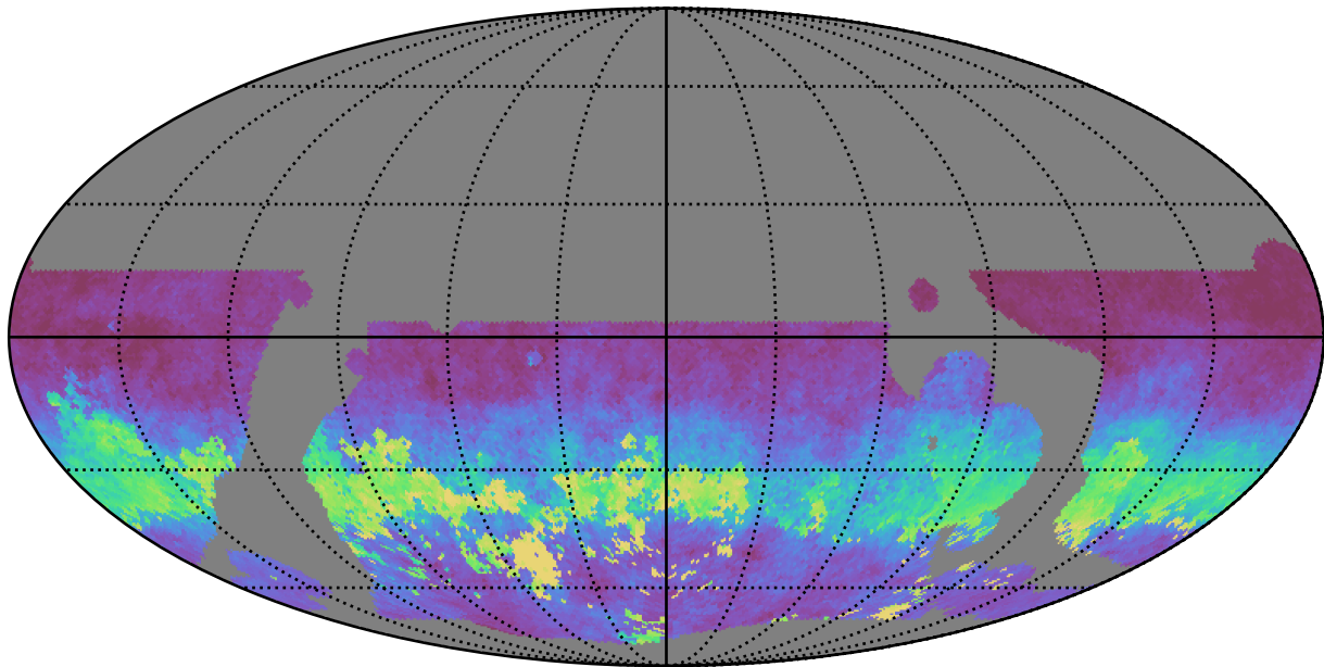
weather_cloudso0v3.5_10yrs WFD g band: AngleRms rotSkyPos
