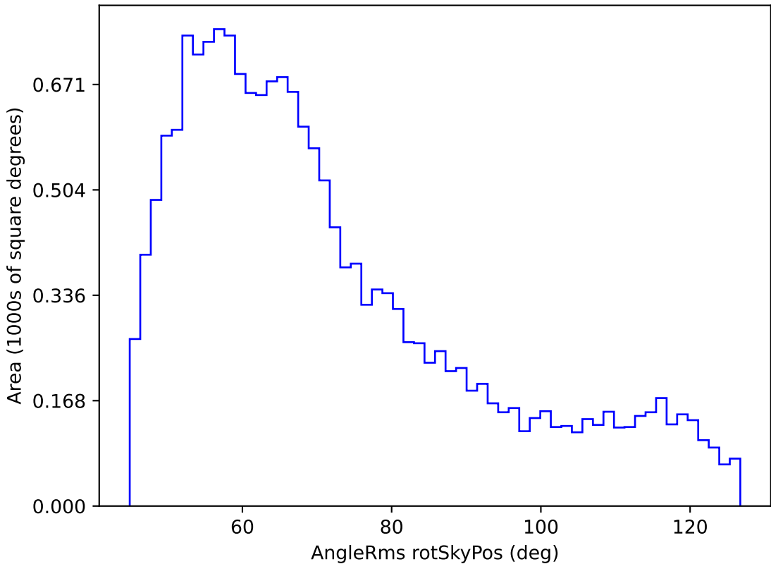
weather_cloudso0v3.5_10yrs WFD g band: AngleRms rotSkyPos
