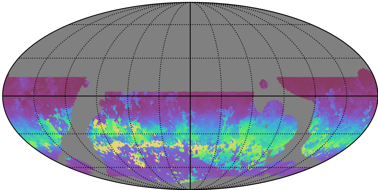
weather_cloudso0v3.5_10yrs WFD all bands: AngleRms rotSkyPos
