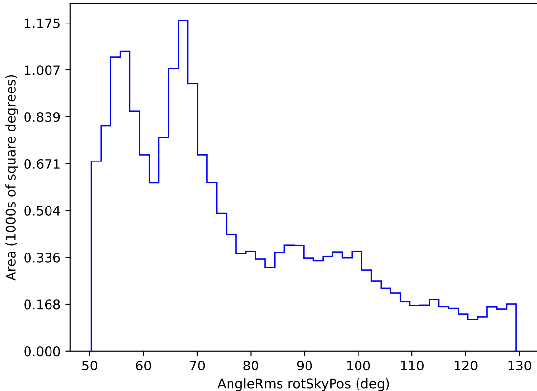
weather_cloudso0v3.5_10yrs WFD all bands: AngleRms rotSkyPos
