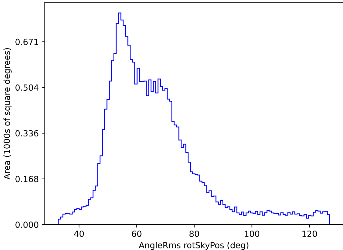
weather_cloudso0v3.5_10yrs All sky y band: AngleRms rotSkyPos
