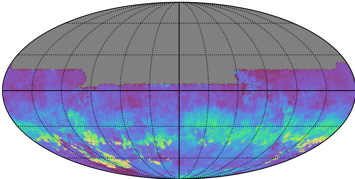
weather_cloudso0v3.5_10yrs All sky u band: AngleRms rotSkyPos
