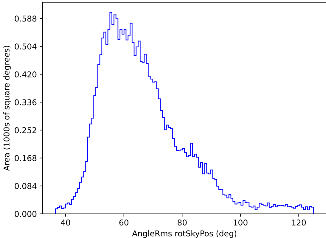
weather_cloudso0v3.5_10yrs All sky u band: AngleRms rotSkyPos
