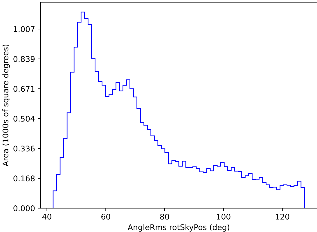
weather_cloudso0v3.5_10yrs All sky r band: AngleRms rotSkyPos
