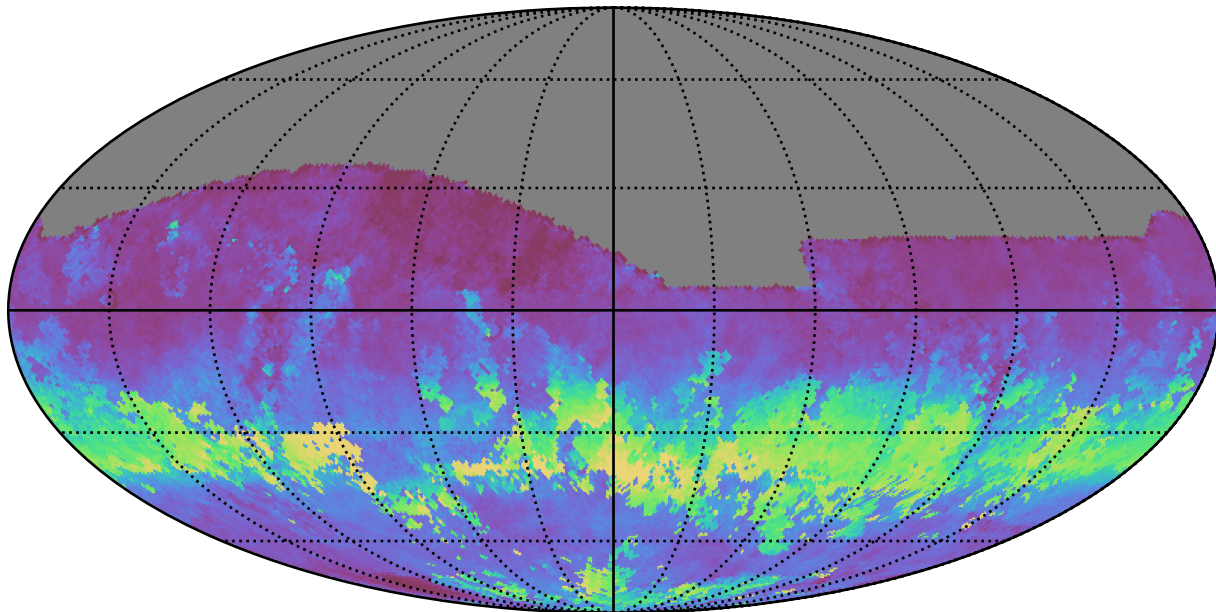
weather_cloudso0v3.5_10yrs All sky i band: AngleRms rotSkyPos
