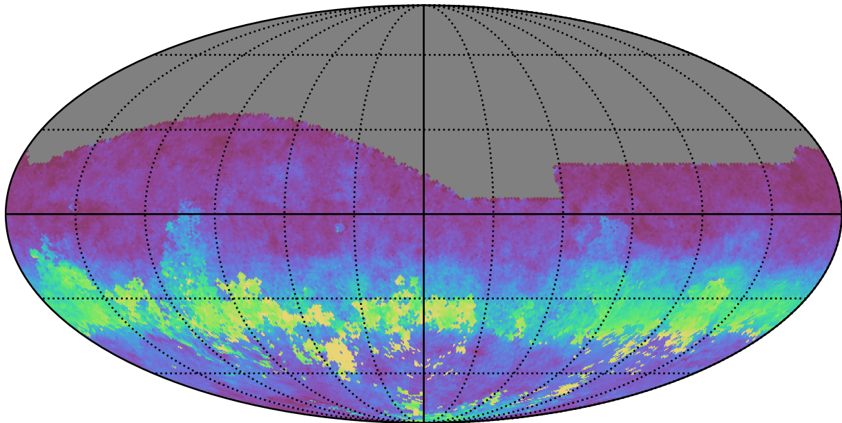
weather_cloudso0v3.5_10yrs All sky g band: AngleRms rotSkyPos
