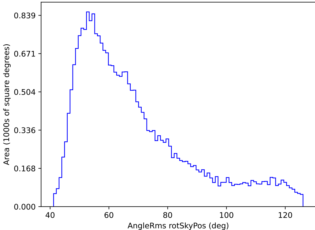
weather_cloudso0v3.5_10yrs All sky g band: AngleRms rotSkyPos
