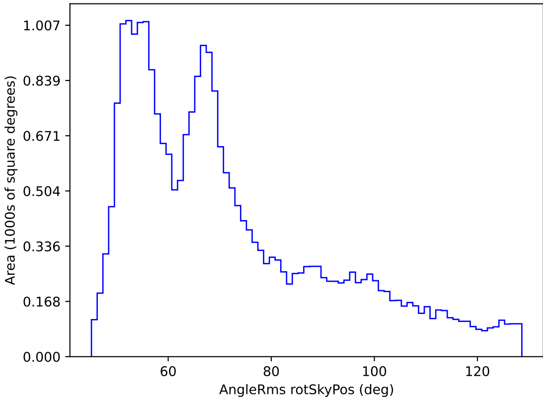
weather_cloudso0v3.5_10yrs All sky all bands: AngleRms rotSkyPos
