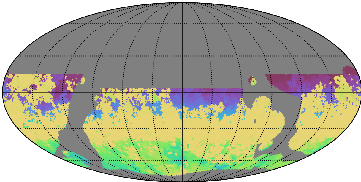
weather_cloudso0v3.5_10yrs WFD all bands: AngleRange rotSkyPos
