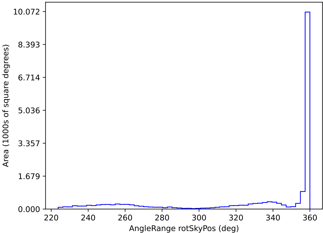
weather_cloudso0v3.5_10yrs WFD all bands: AngleRange rotSkyPos
