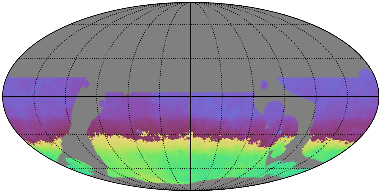
weather_cloudso0v3.5_10yrs WFD z band: AngleMean rotSkyPos
