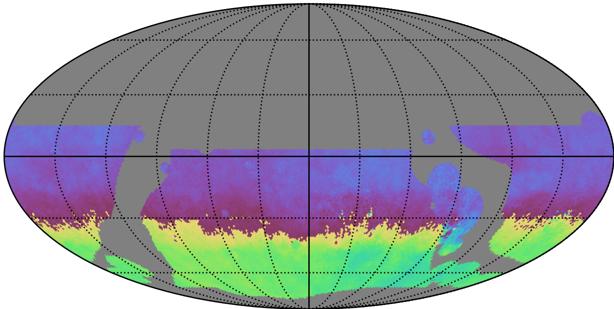
weather_cloudso0v3.5_10yrs WFD u band: AngleMean rotSkyPos
