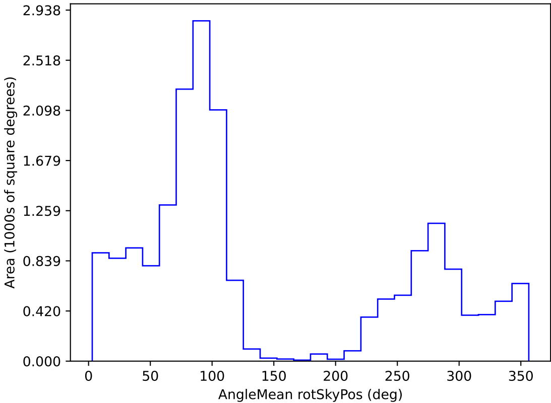
weather_cloudso0v3.5_10yrs WFD u band: AngleMean rotSkyPos
