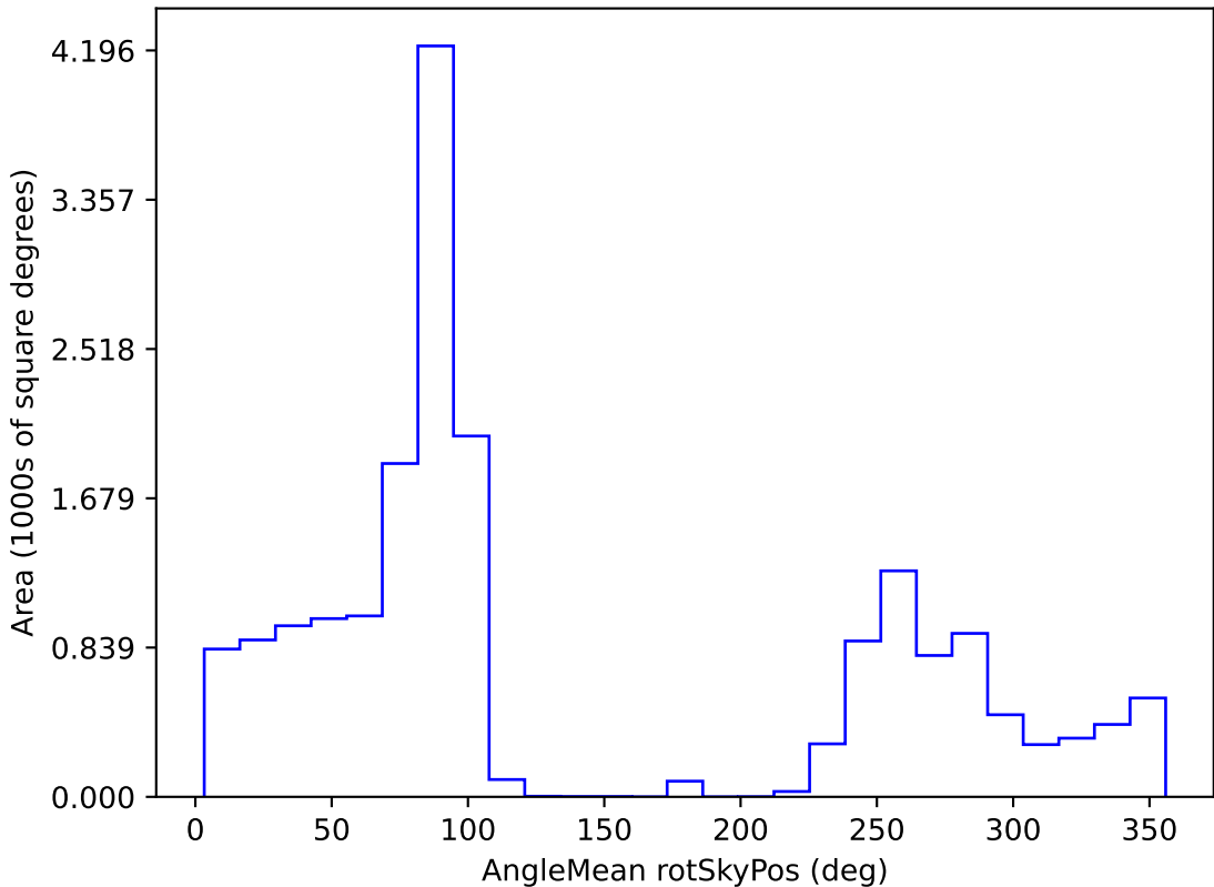
weather_cloudso0v3.5_10yrs WFD r band: AngleMean rotSkyPos
