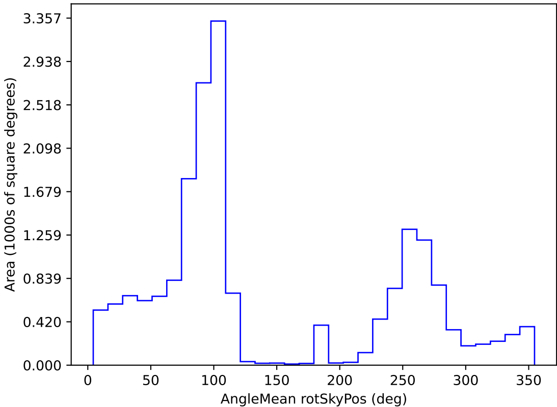
weather_cloudso0v3.5_10yrs WFD g band: AngleMean rotSkyPos
