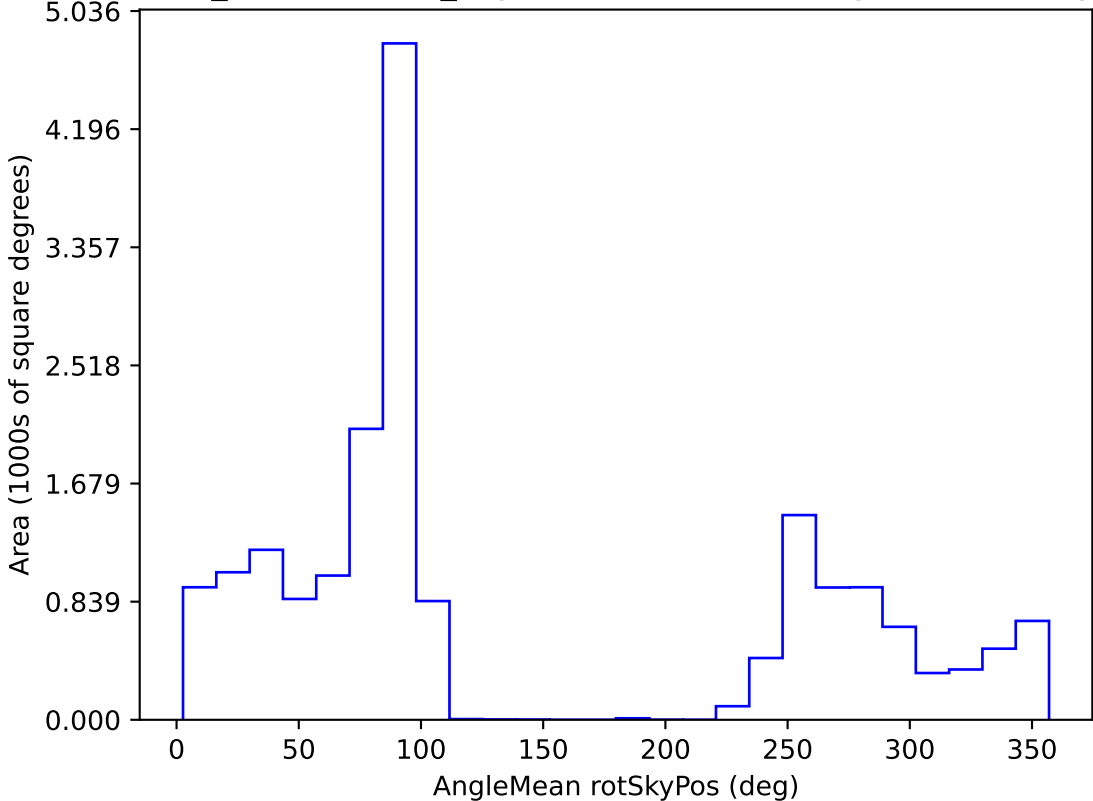
weather_cloudso0v3.5_10yrs WFD all bands: AngleMean rotSkyPos
