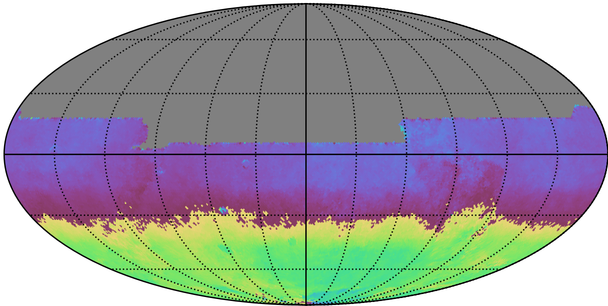
weather_cloudso0v3.5_10yrs All sky y band: AngleMean rotSkyPos
